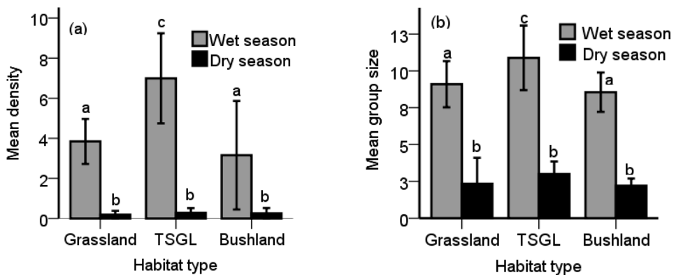
Fig. 2. Seasonal mean density (a) and group size (b) of Beisa oryx in the Alledoghi Wildlife Reserve. Means indicated by different letters in each figure are significantly different at \alpha = 0.05 (TSGL = wooded grassland).
