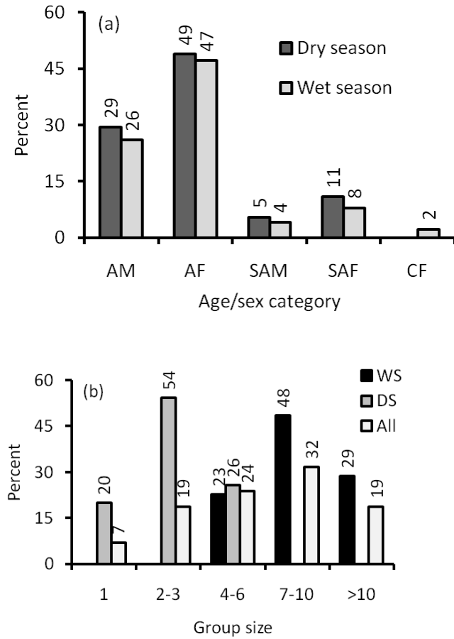
Fig. 3. Percentage contribution of each age/sex category to the total population (a) and group size frequency (b) of Beisa oryx in Alledoghi Wildlife Reserve during the wet and dry seasons. Sample size (N) for age/sex category, = 732 during wet season, and 92 during dry season; for group size, = 66 in wet season, = 35 in dry season, = 101 total. (Abbreviations, age/sex category: AM = adult male, AF = adult female, SAM = sub-adult male, SAF = sub-adult female, CF = calf).
